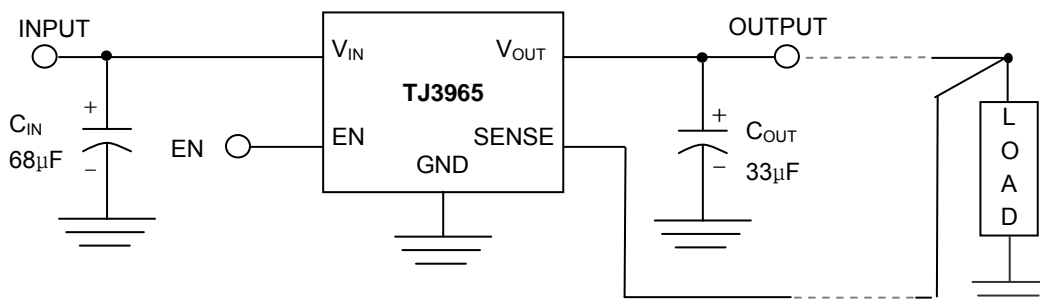
5 / 8 Pin Remote Load Sense Application
