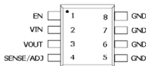
SOP8 / SOP8-PP
