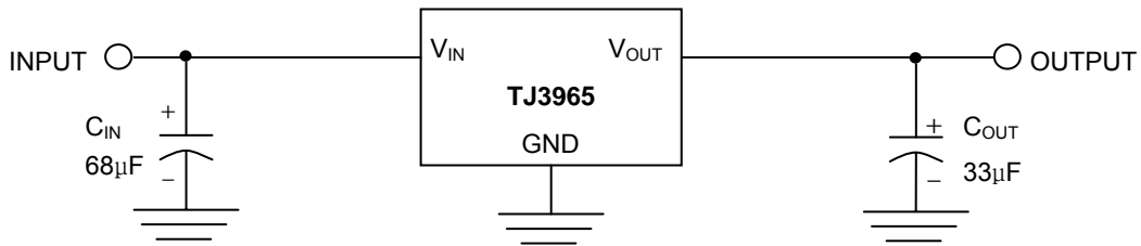
Typical 5 / 8 Pin Application
