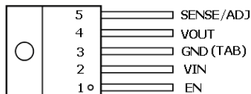
TO220-5L
