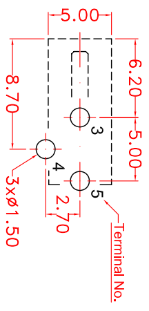
PIERCING PLAN
