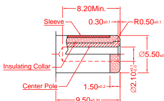
Mate Plug
