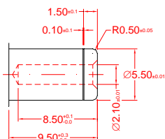
Gauge Plug
