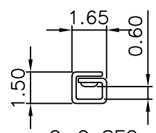
C-C SEC
