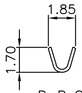
B-B SEC
