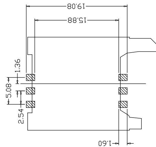
REFERENCE PC BOARD LAYOUT
